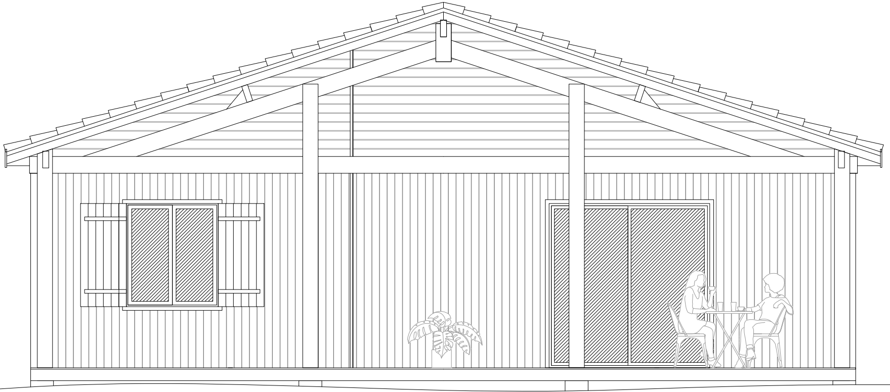
FACADE SUD
